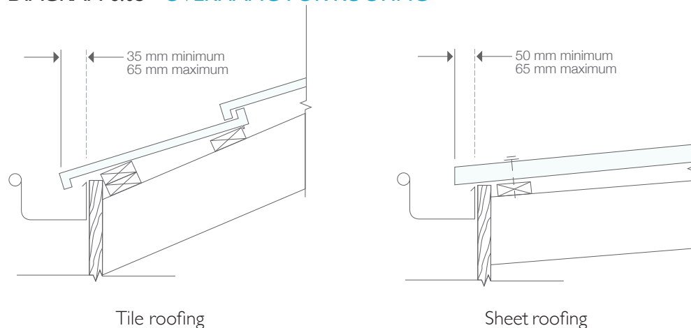
DIAGRAM 6.05 OVERHANG FOR ROOFING
