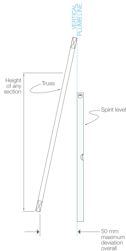
DIAGRAM 6.10 VERTICALITY OF TRUSSES
